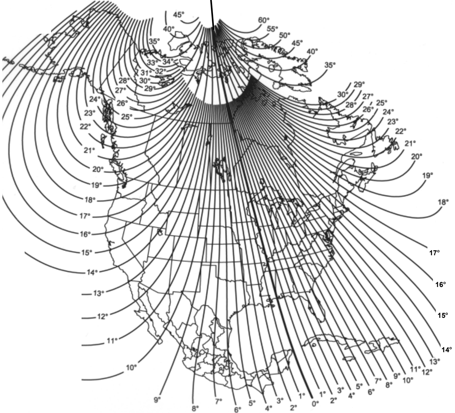
LINES OF EQUAL MAGNETIC DECLINATION 2000
