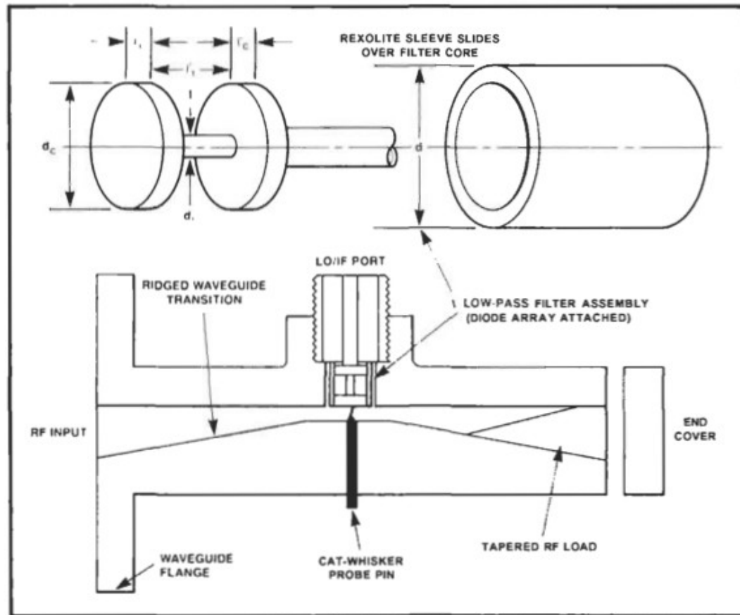
Figure 10. Millimetric mixer construction.
